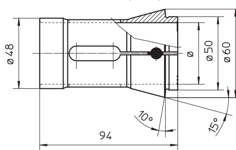
liscia (HTK-TL) round-smooth collet (HTK-TL)
