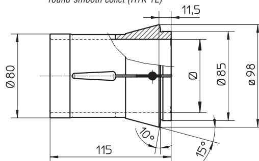
liscia (HTK-TL) round-smooth collet (HTK-TL)
